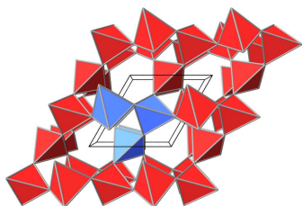
alpha-Quarz (Polyederdarst.)
