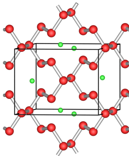
\text{BaSb}_3
