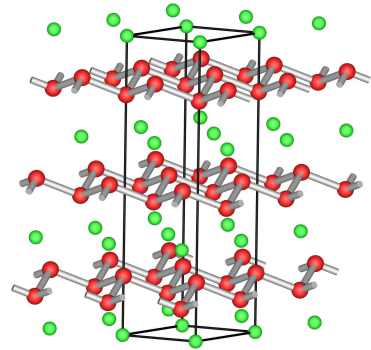
\text{CaSi}_2
