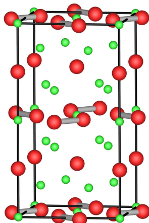
\text{Ca}_5\text{Si}_3
