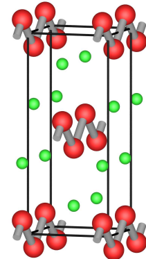
\text{CaSi}
