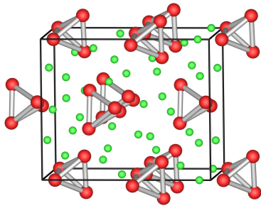
\text{Na}_2\text{Tl}
