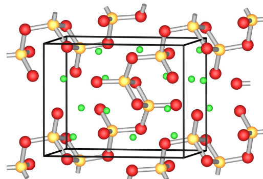
\text{Na}_7\text{In}_3\text{Se}_8
