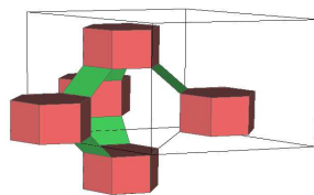
Gmelinit (Polyeder)
