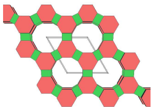
Gmelinit
