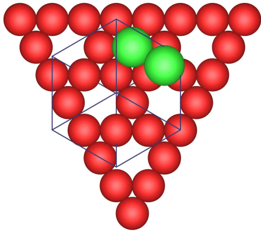
Cu-Kagome-Netz
